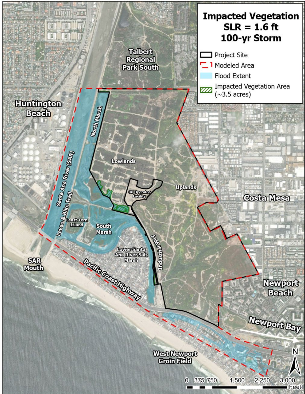
FIGURE 40: IMPACTED VEGETATION (1.6 FT SLR, 100-YEAR STORM)
