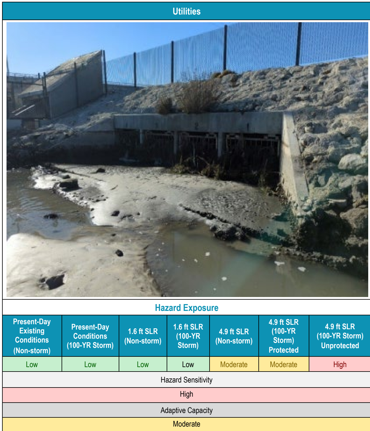
FIGURE 47: HAZARD EXPOSURE, HAZARD SENSITIVITY, & ADAPTIVE CAPACITY: UTILITIES
