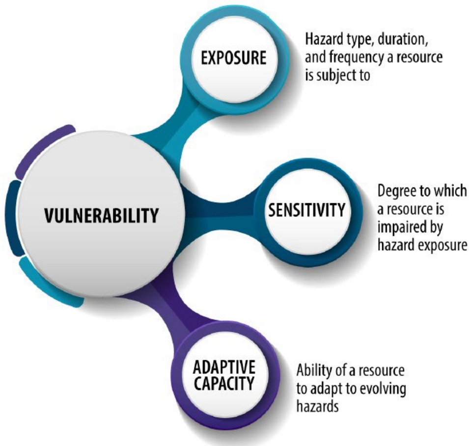
FIGURE 36: COMPONENTS OF SEA LEVEL RISE VULNERABILITY AS DEFINED WITHIN THIS STUDY
