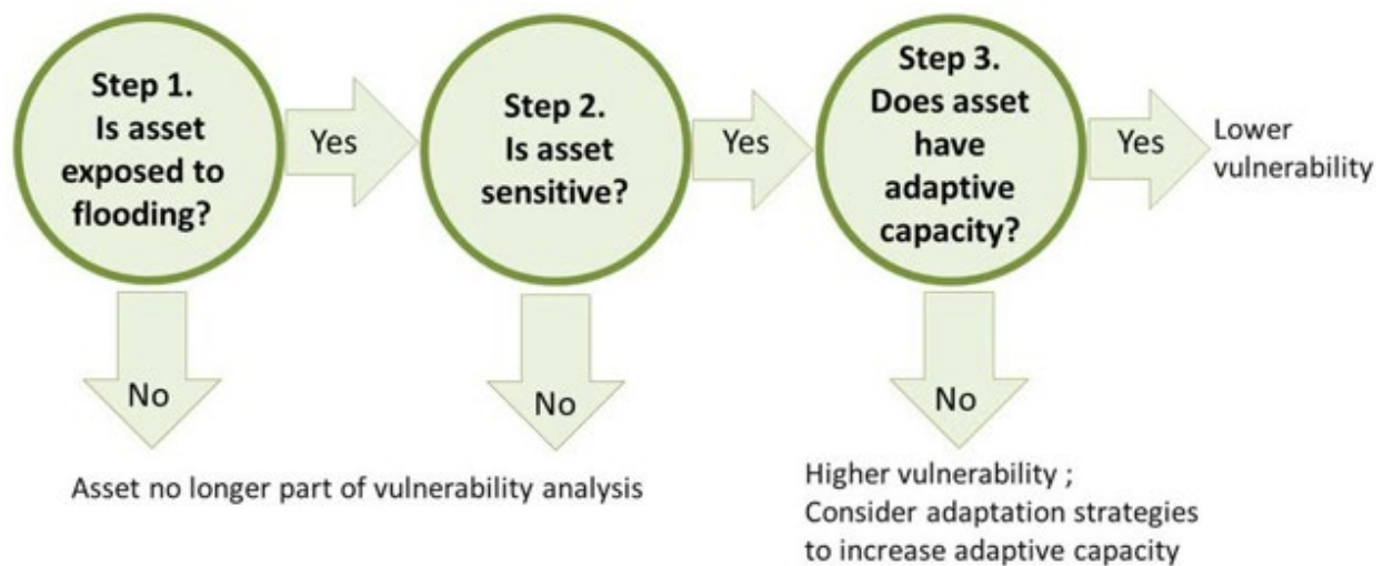
FIGURE 44: STEPWISE ROADMAP OF VULNERABILITY ANALYSIS
