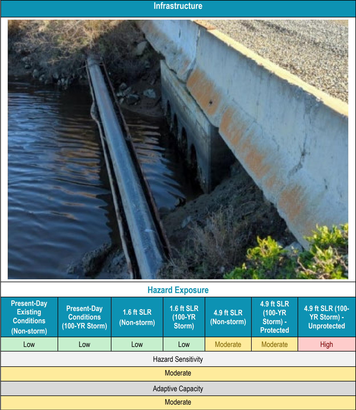
FIGURE 48: HAZARD EXPOSURE, HAZARD SENSITIVITY, & ADAPTIVE CAPACITY: INFRASTRUCTURE
