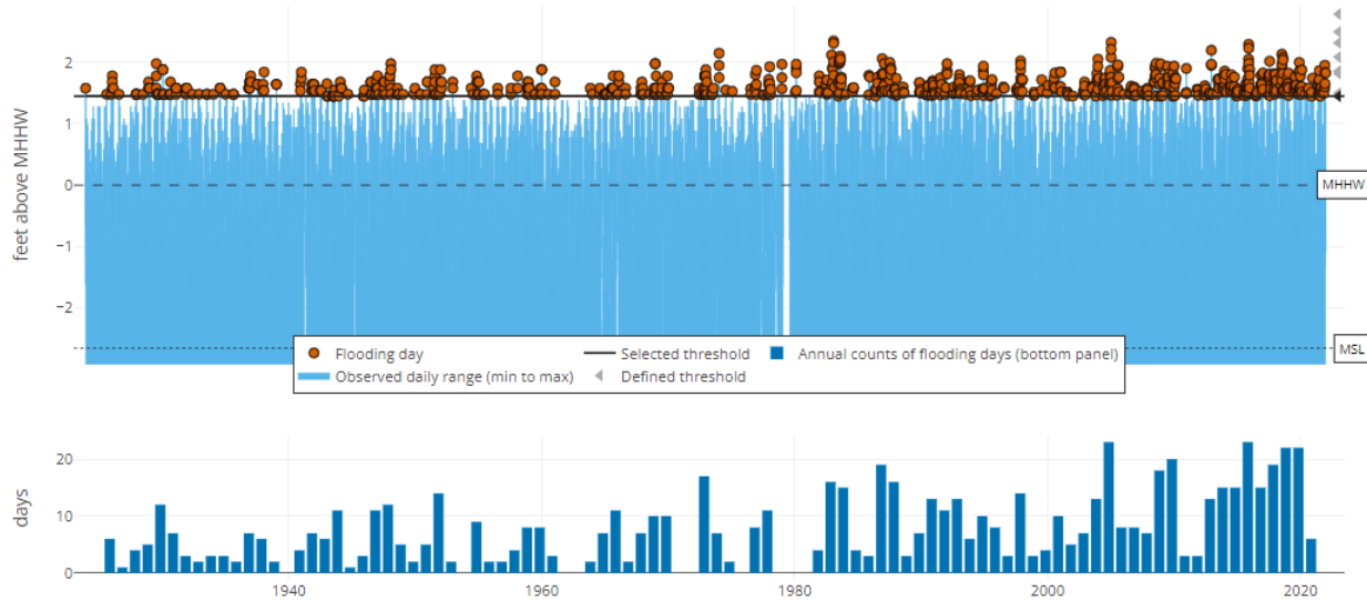
FIGURE 27: OBSERVED FLOODING DAYS AT NOAA STATION 9410660 (LOS ANGELES) FOR 1-YEAR FLOOD THRESHOLD
